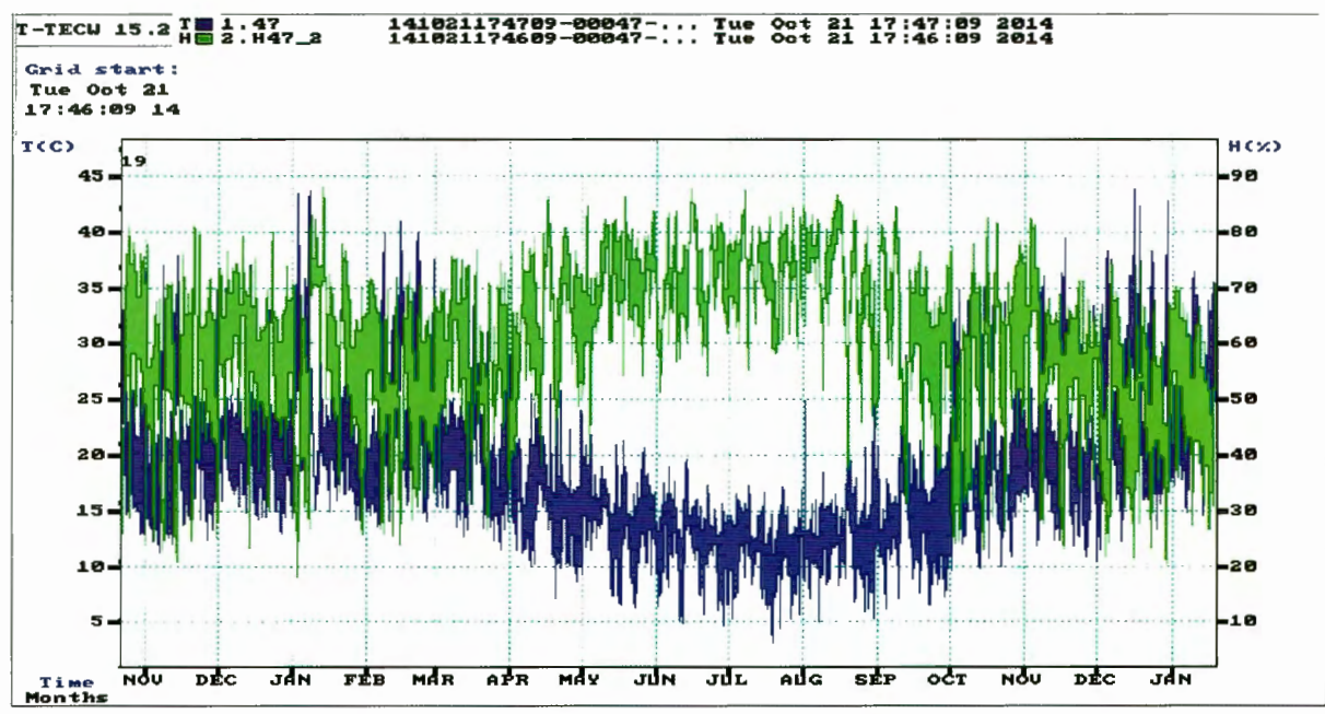
Outdoor temperature and humidity in Adelaide – from wireless T-TEC logger in wrap-around mode. The file has 1.3 million logs, collected in the database.
